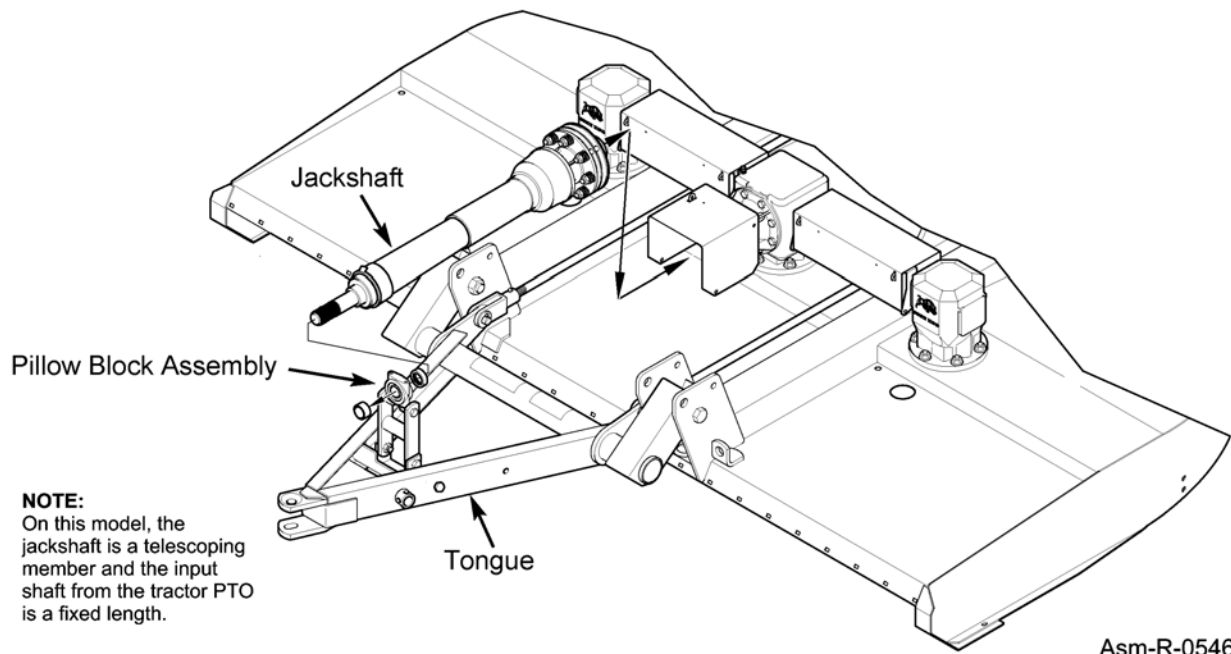
Pull Model with Pillow Block and Jackshaft
