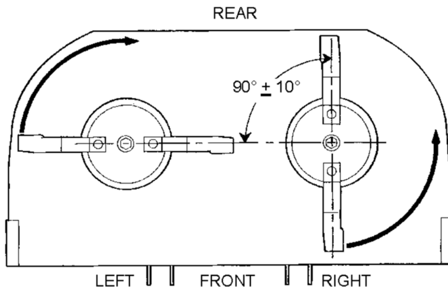
Blade Pan Timing As Viewed From Bottom Of Cutter
