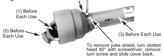
BINACCHI DRIVELINE (2) Before Each Use
