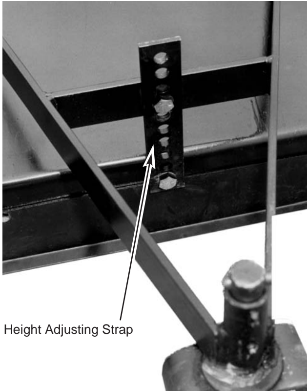
Figure 3-1 Cutting Height Adjustment
