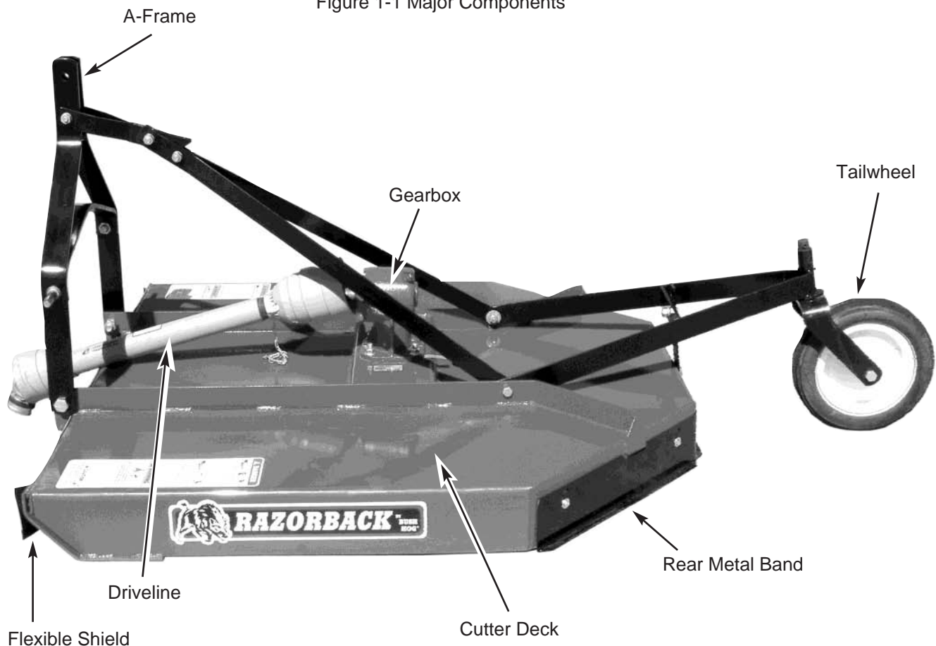
Figure 1-1 Major Components
