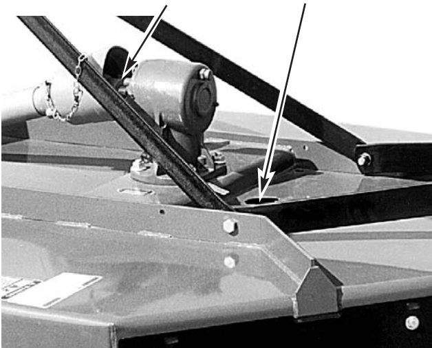
Figure 4-3 Shear Bolt Blade Bolt
