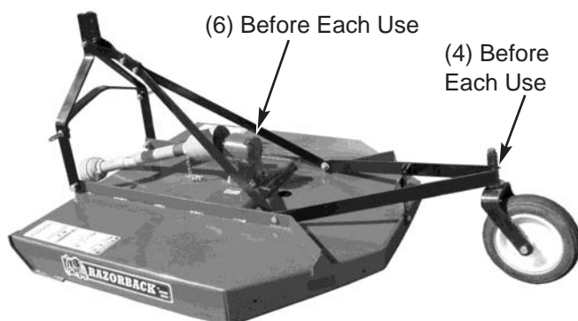
Figure 4-1 Lubrication
