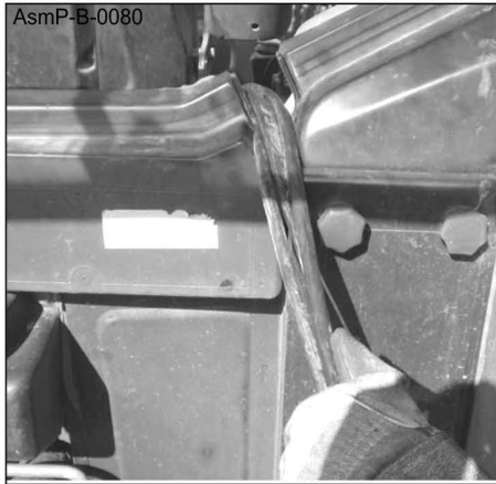
Feed control lines into tractor cab avoid sharp bends and keep lines well clear of all moving parts on the machine or tractor.
