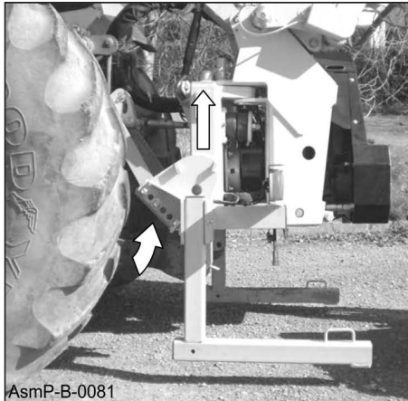
Tighten tractor stabilizers raise tractor linkage to lift the machine to its working height.
